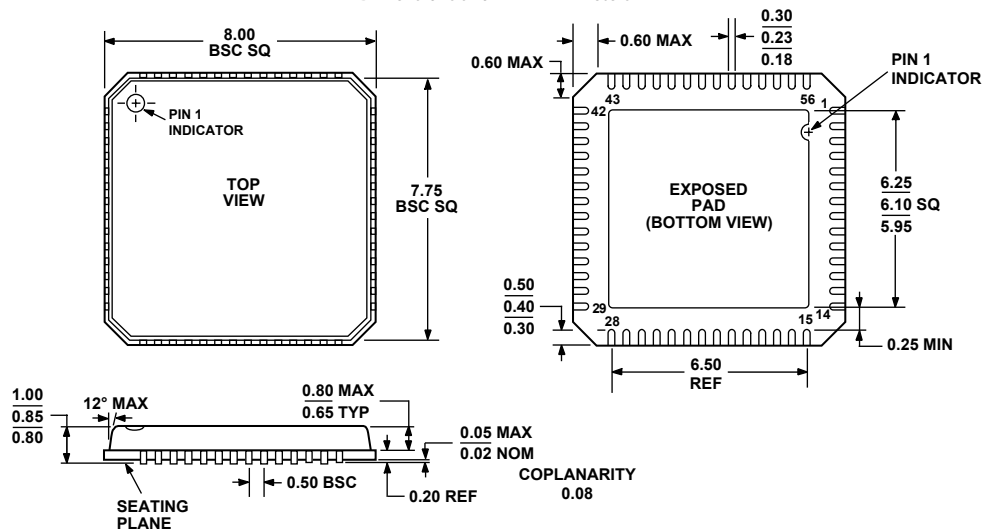
Figure 27. 56-Lead Lead Frame Chip Scale Package (CP-56-1)
