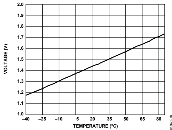
Figure 19. TEMP\_OUT Voltage vs Temperature
