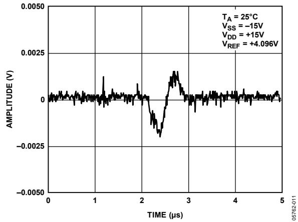
Figure 12. Digital Crosstalk
