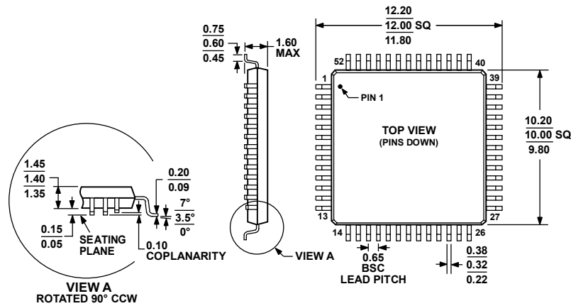
Figure 26. 52-Lead Low Profile Quad Flat Package [LQFP] (ST-52)
