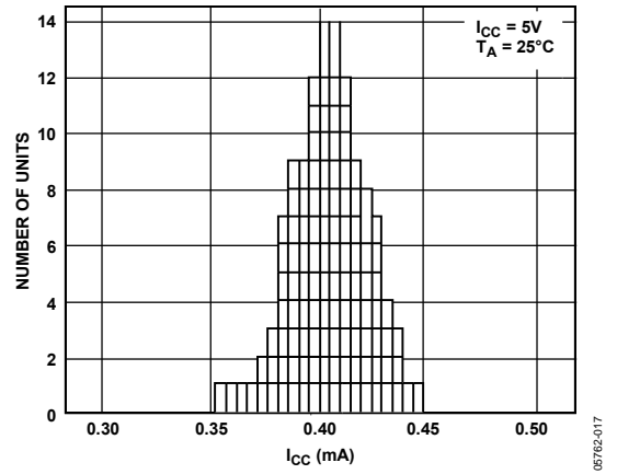
Figure 18. Typical I_{CC} Distribution
