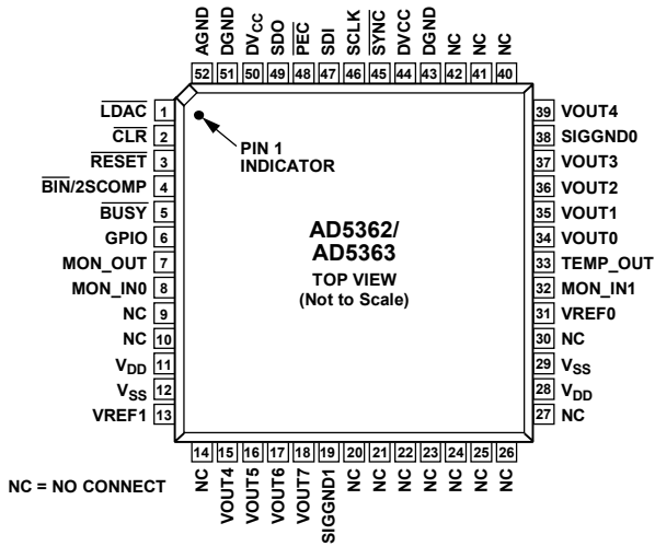
Figure 7. LQFP Pin Configuration
