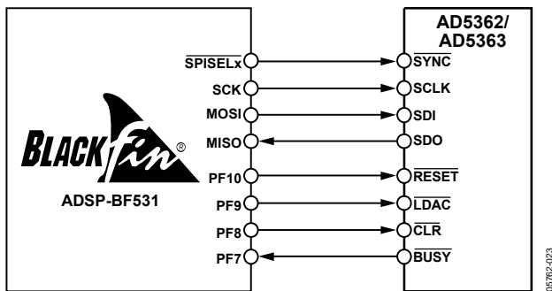
Figure 24. Interfacing to a Blackfin DSP
