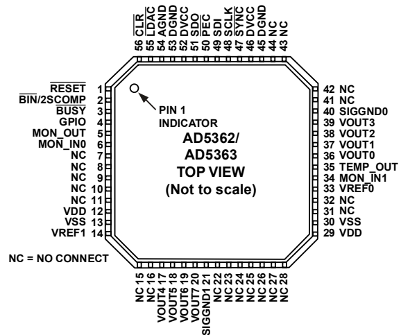
Figure 8. LFCSP Pin Configuration
