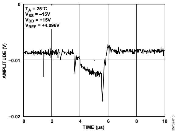
Figure 11. Analog Crosstalk Due to \overline{LDAC}
