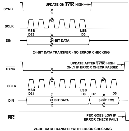
5360-0010 Figure 11. SPI Write With and Without Error Checking
